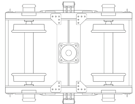
Bogie Commonwealth On30.
